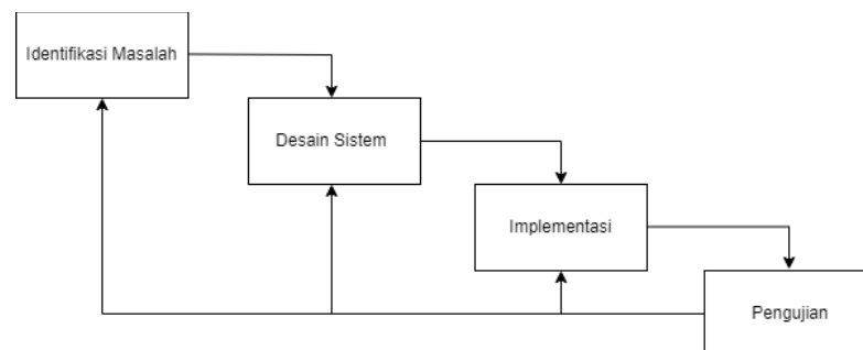
Gambar 3. 1 Flowchart Penelitian
