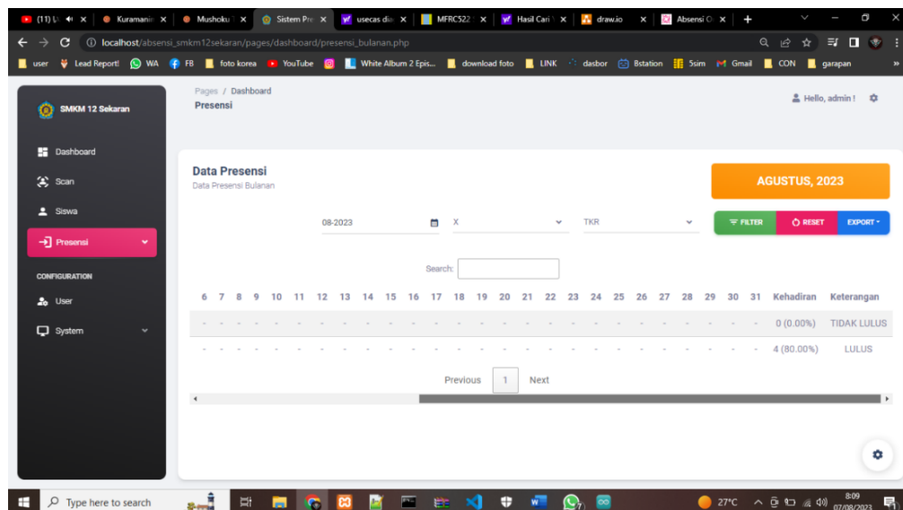
Gambar 4. 20 Perhitungan Absensi
