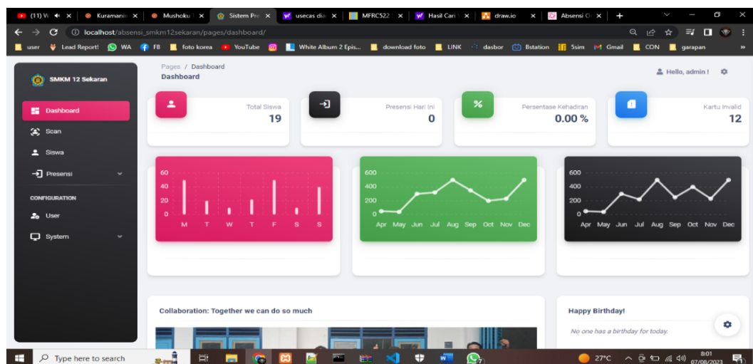
Gambar 4. 12 Dashboard
