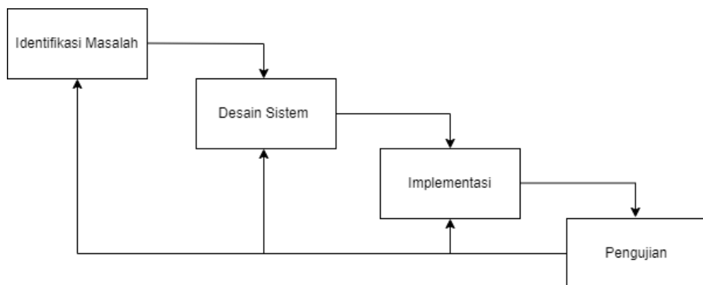
Gambar 2. 9 Metode Waterfall
