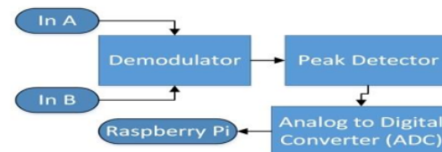
Fig. 4: Voltage Measurement Diagram.
