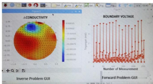
Fig. 9: Graphics User Interface (GUI) for the Manufactured EIT.
