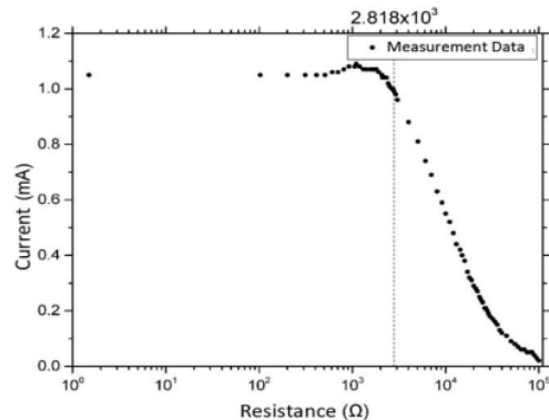
Fig. 8: VCCS Load Ranging from 1 – 100 K \Omega That Used to Conduct Test the Ability of EIT for Supporting High Impedance Tissue.
