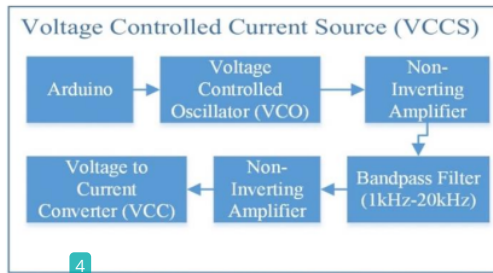
Fig. 2: Voltage Controlled Current Source (VCCS) Circuit Design.
