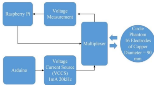
Fig. 1: Design of Electrical Impedance Tomography with the High-Speed System.
