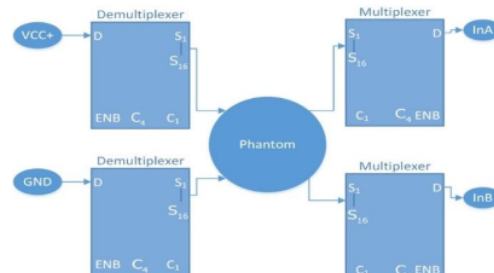
Fig. 3: Multiplexer/Demultiplexer Design for High-Speed EIT System.
